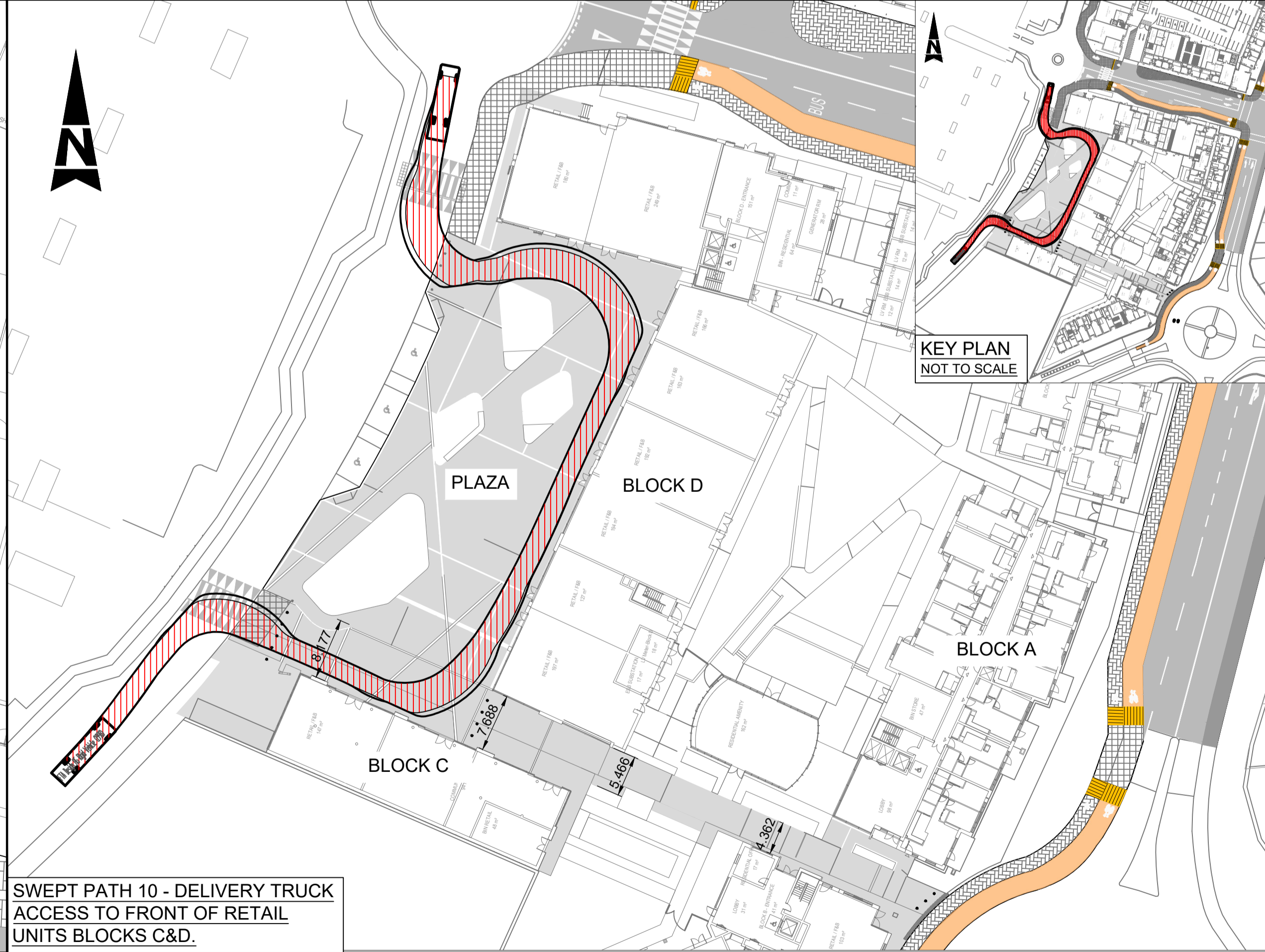
KEY PLAN NOT TO SCALE SWEPT PATH 9 - DELIVERY TRUCK FOR RETAIL IN BLOCK E
